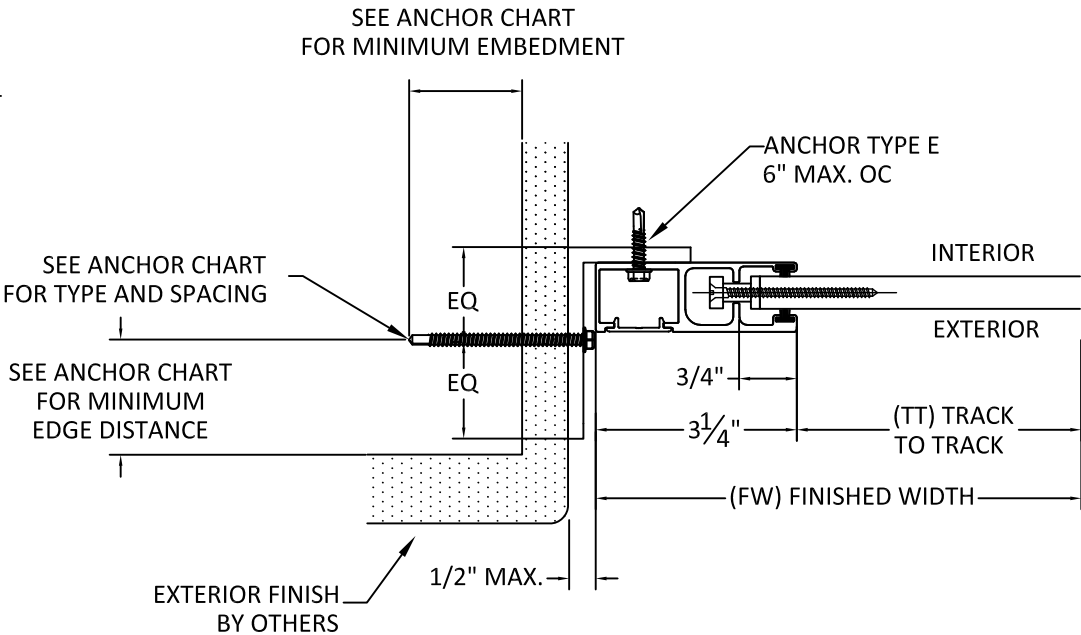
H1 8 HORIZONTAL SECTION MOUNT TYPE 3 - ALTERNATE INSET MOUNT *WITH END RETENTION
